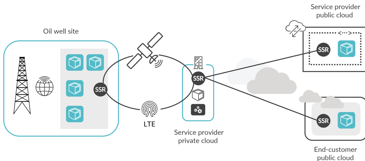
Figure 1: Next-Generation digital oil field with AI-Driven SD-WAN
