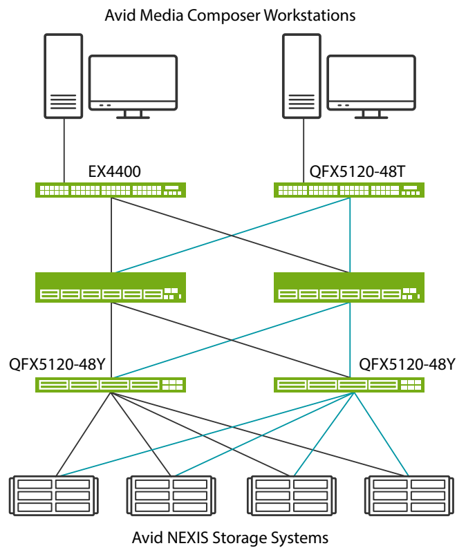
Figure 1: Avid reference architecture with Juniper switches. The QFX5120 Switch connects to Avid NEXIS storage and both QFX5120 switches and the Juniper Networks EX4400 Ethernet Switch connect to Avid Media Composer clients
