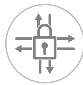
SD-WAN Security
