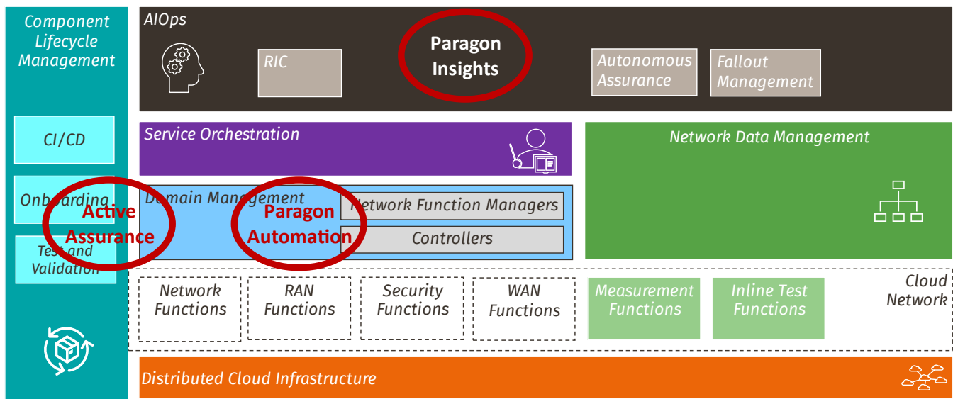
Figure 1: Paragon Automation integrates assets from across the NAS taxonomy
